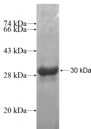
Recombinant Human CUL4B SDS-PAGE
