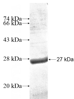
Recombinant Human C1orf57 SDS-PAGE
