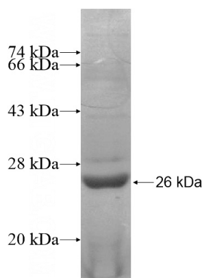
Recombinant Human TMEM177 SDS-PAGE
