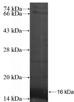
Recombinant Human ATAD4 SDS-PAGE
