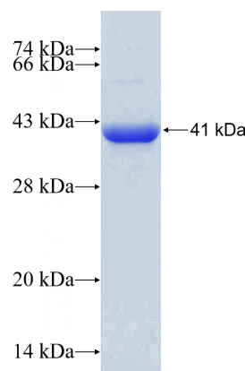
Recombinant Human GAPDH SDS-PAGE
