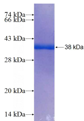
Recombinant Human MRPS18B SDS-PAGE
