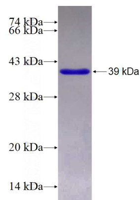
Recombinant Human CHMP4C SDS-PAGE
