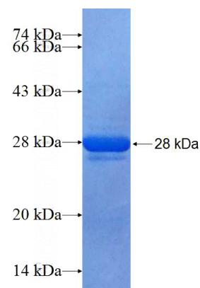
Recombinant Human MRPS26 SDS-PAGE
