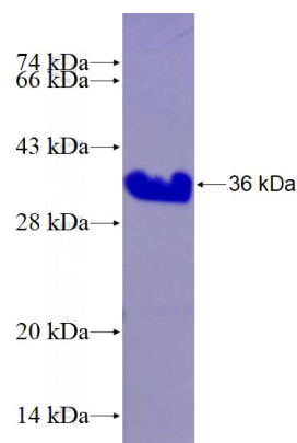
Recombinant Human SLC4A1 SDS-PAGE
