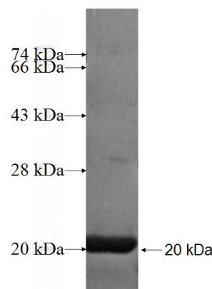
Recombinant Human PFDN6 SDS-PAGE
