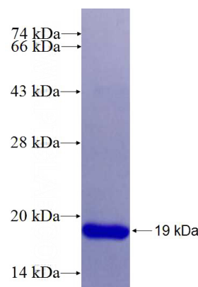
Recombinant Human AP50 SDS-PAGE
