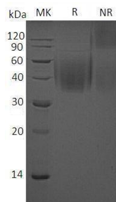
Mouse Cd244/2b4/Nmrk (His tag) recombinant protein
