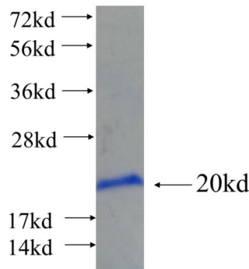
Recombinant human ZNF549 SDS-PAGE
