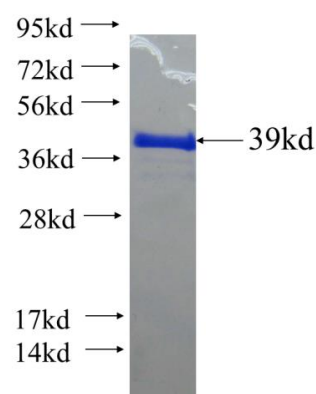
Recombinant human ZNF48 SDS-PAGE
