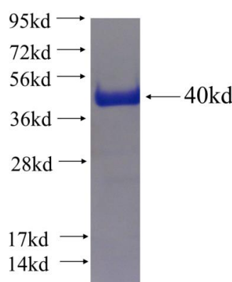
Recombinant human ZFYVE28 SDS-PAGE
