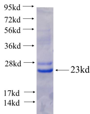
Recombinant human ZAP70 SDS-PAGE
