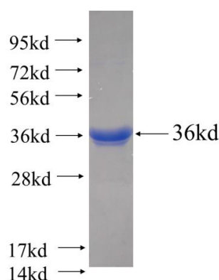
Recombinant human UQCRFS1(Full length) SDS-PAGE
