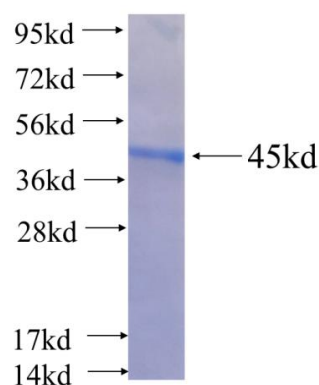
Recombinant human UGT2B4 SDS-PAGE
