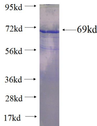
Recombinant human TYW1B SDS-PAGE
