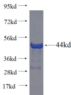
Recombinant human TTC28 SDS-PAGE
