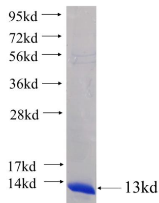
Recombinant human TMSB4X(Full length) SDS-PAGE
