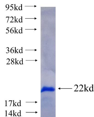
Recombinant human THAP2 SDS-PAGE
