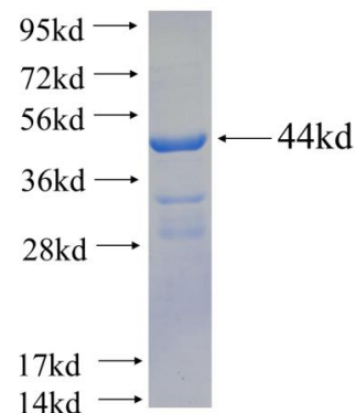
Recombinant human TBC1D17 SDS-PAGE
