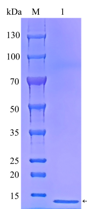
Recombinant human SV2C SDS-PAGE
