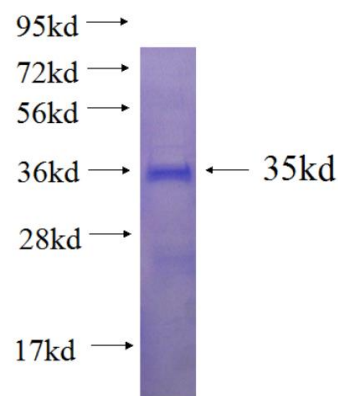
Recombinant human SUV39H1 SDS-PAGE
