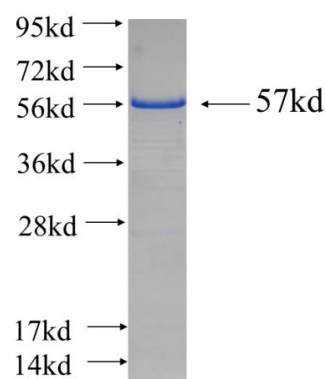
Recombinant human SUPT5H SDS-PAGE
