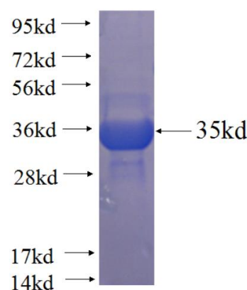
Recombinant human SPANXN4 SDS-PAGE
