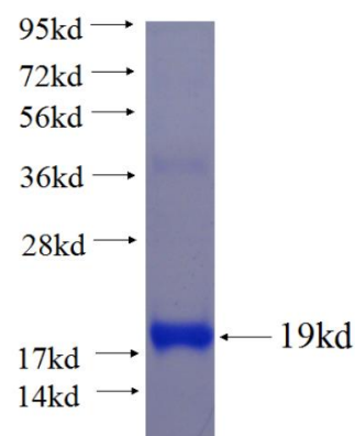
Recombinant human SLC16A9 SDS-PAGE
