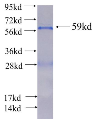
Recombinant human SH3GL3(Full length) SDS-PAGE
