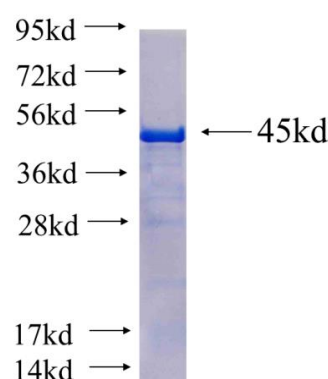
Recombinant human SH3D19 SDS-PAGE
