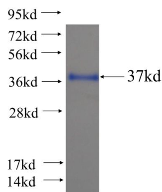
Recombinant human RRN3 SDS-PAGE
