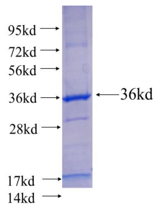
Recombinant human RPL7A(Full length) SDS-PAGE
