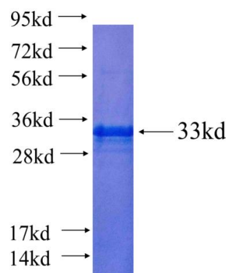
Recombinant human RLBP1L2 SDS-PAGE
