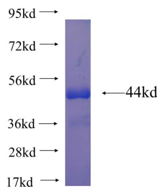
Recombinant human PUM2 SDS-PAGE
