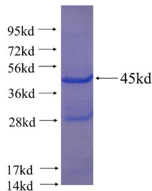
Recombinant human NAT5 SDS-PAGE
