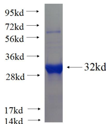
Recombinant human MT2A SDS-PAGE
