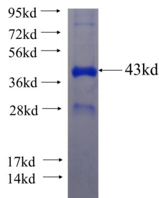
Recombinant human MGAT1 SDS-PAGE
