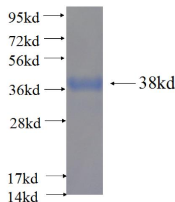
Recombinant human LRRFIP1 SDS-PAGE
