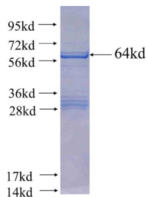
Recombinant human LGALS12(Full length) SDS-PAGE
