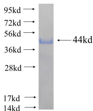
Recombinant human KCNA2 SDS-PAGE
