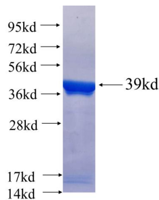
Recombinant human IWS1 SDS-PAGE
