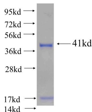
Recombinant human HNRNPH3 SDS-PAGE
