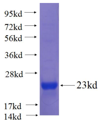
Recombinant human GALNT9 SDS-PAGE
