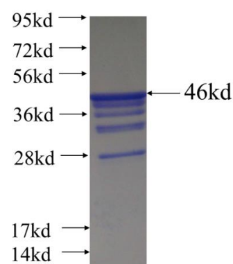
Recombinant human FMR1 SDS-PAGE
