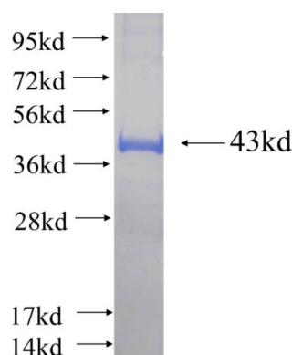
Recombinant human FGD3 SDS-PAGE
