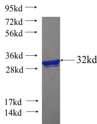
Recombinant human FBP2 SDS-PAGE
