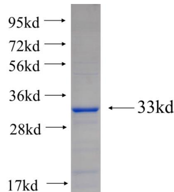
Recombinant human FAM181A SDS-PAGE
