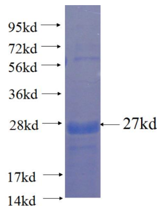
Recombinant human FAM110B SDS-PAGE
