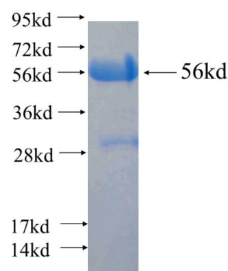
Recombinant human EXOSC8(Full length) SDS-PAGE
