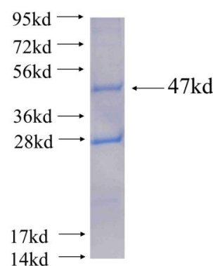
Recombinant human CRYGC(Full length) SDS-PAGE
